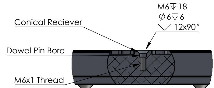
DETAIL B 3-IN-1 FIXTURING LOCATOR SCALE 1 : 2
