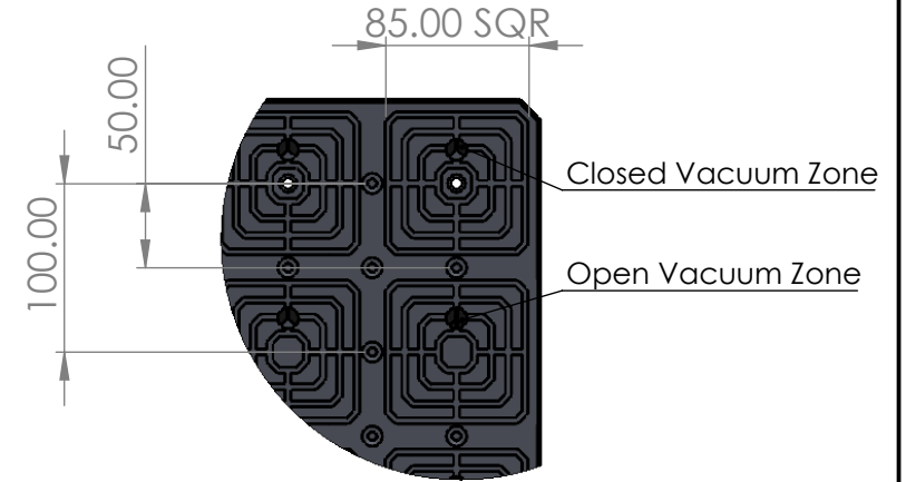
DETAIL A VACUUM ZONES SCALE 1 : 5
